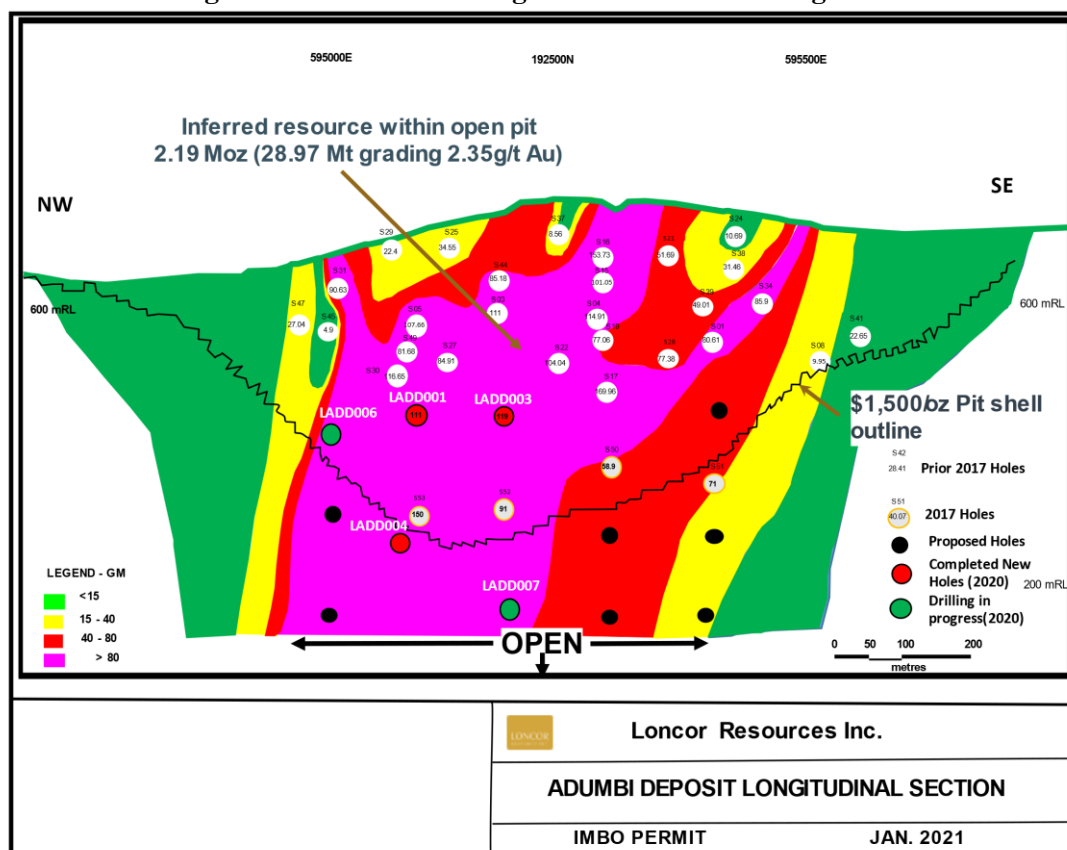
Figure 2: Adumbi Longitudinal Section Looking Northeast with Drilling Pierce Points
